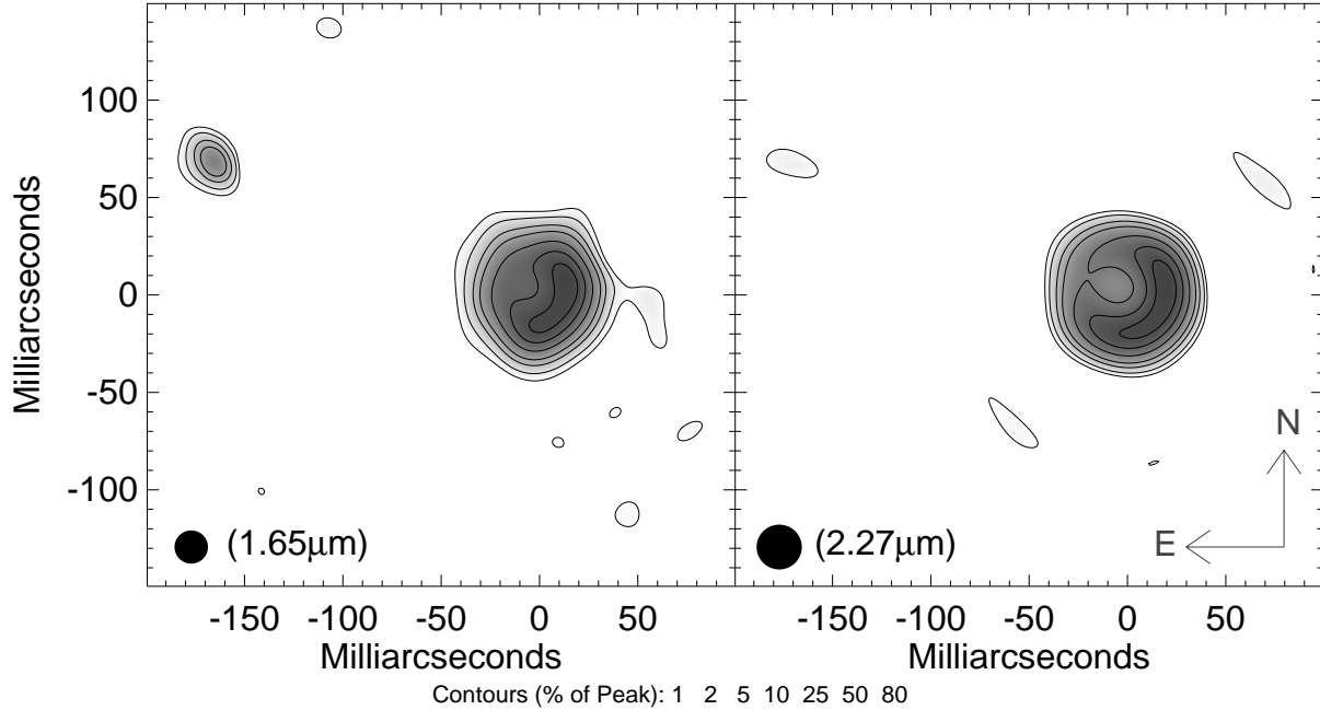
Figure 1: Maps of the LkH \alpha 101 system. Maximum-Entropy image reconstructions at 1.65 (left) and 2.27 \mu\text{m} (right) from data taken in September 1998 (JD 2451086). Filter bandwidths were 0.33 and 0.16 \mu\text{m} respectively. As it is difficult to extract both absolute astrometry and photometry with our interferometric techniques, the origin has been centered on the disk and images scaled to the brightest pixel. The K-band map is of slightly superior quality to H-band due to the less-detrimental impact of the seeing at longer wavelengths. High spatial resolution information was extracted from high magnification (20 mas/pixel) fast-readout ( \sim 130 ms) data frames taken with an annulus-shaped aperture mask[16]. Consecutive sets of 100 images, interleaved between LkH \alpha 101 and nearby point-source objects, allowed calibration of the statistical behavior of the telescope-atmosphere point-spread function. Data were processed to extract Fourier bispectral data, with the final output being a calibrated set of 630 Fourier amplitudes and 7140 closure phases. High-quality images were produced from an algorithm based on the maximum entropy method[26, 27], although other methods such as CLEAN have also been utilized with near-identical results. The fidelity of our mapping process has been extensively tested on binary stars and other known compact asymmetric targets[28, 29].
