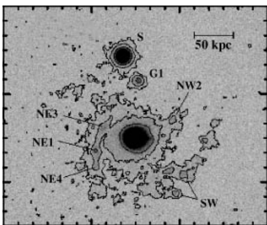
A NEARBY ( z = 0.06 ) QUASAR, imaged with the Taurus Tunable Filter at the 3.9m Anglo-Australian Telescope. A gas envelope 600,000 light years across, companion galaxy, and spiral arms are shown with unusual clarity in the light of ionized hydrogen gas. Credit: Patrick Shoppell
