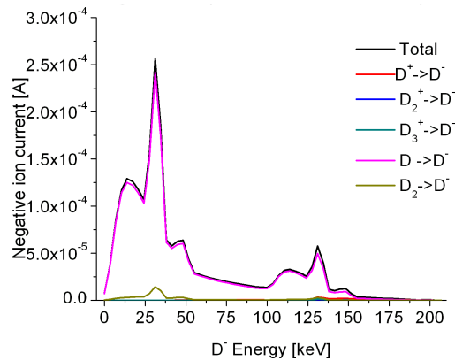
Negative ion spectra from each parent species
