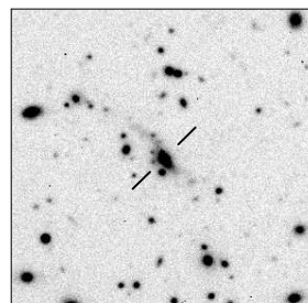
MRC B0511-484
