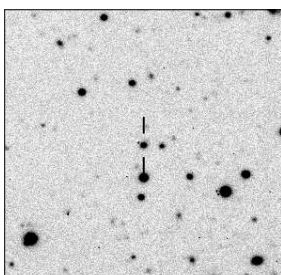
MRC B0547-408
