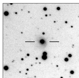
PKS B0707-35
