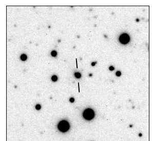
MRC B0842-754
