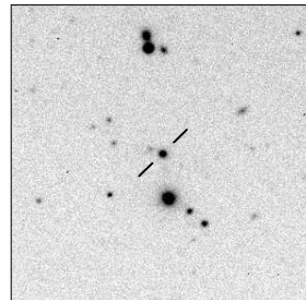
MRC B0357-371
