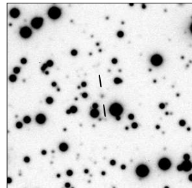
MRC B0910-636
