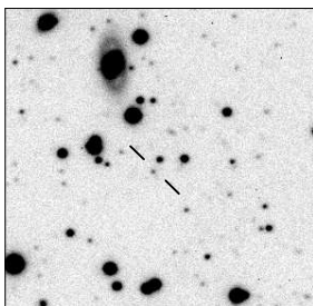
MRC B1232-416
