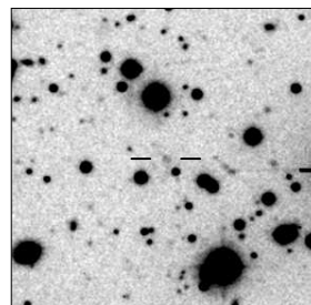
MRC B1247-401
