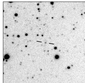
MRC B1206-337
