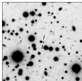
MRC B1234-504
