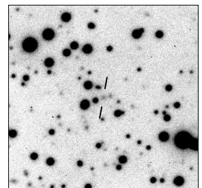
MRC B1259-769
