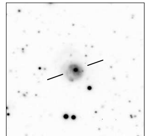
MRC B1221-423
