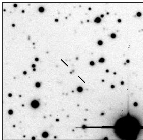
MRC B1003-415
