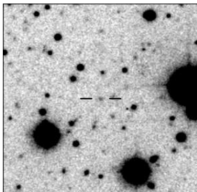
MRC B1143-316
