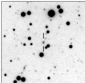
MRC B0842-835
