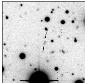
MRC B0846-811
