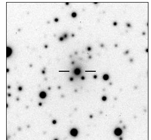
MRC B0943-761
