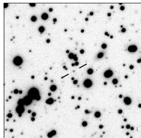
MRC B1036-697
