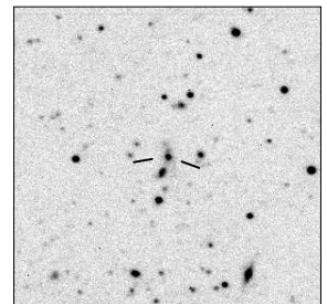
MRC B1136-320
