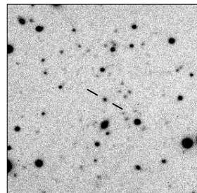
MRC B1044-357
