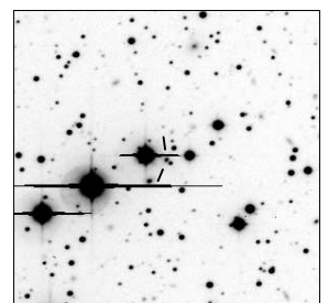
MRC B1737-575
