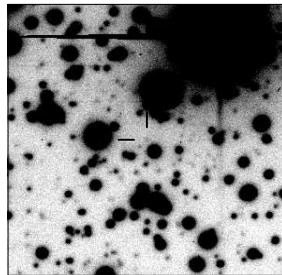
MRC B1421-490
