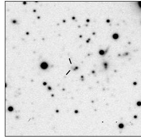
MRC B1346-391
