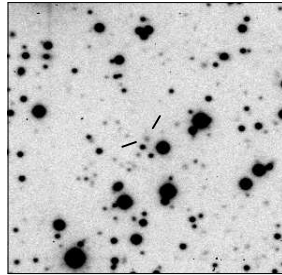
MRC B1315-460
