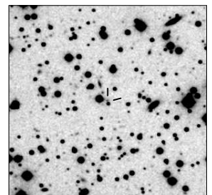
MRC B1633-681
