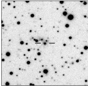
MRC B1259-445
