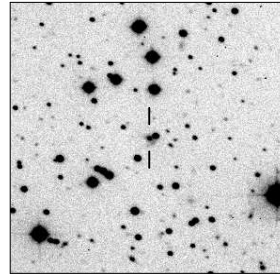
MRC B1817-640
