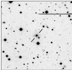
MRC B1819-673
