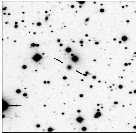
MRC B1737-609
