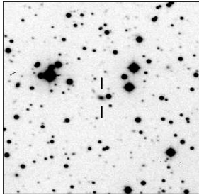
MRC B1814-519
