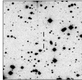
MRC B1754-597
