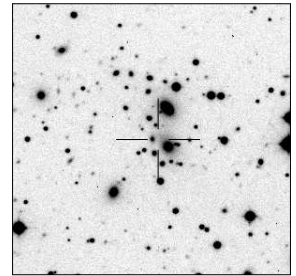
MRC B1917-546
