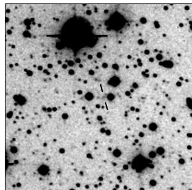
MRC B1923-328
