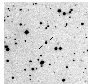
MRC B1933-587
