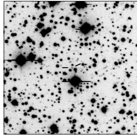
MRC B1817-391
