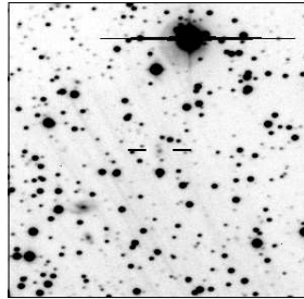
MRC B1740-517
