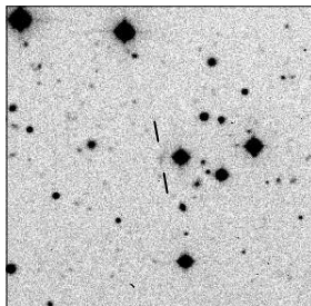
MRC B2226-386
