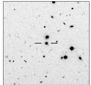
MRC B2122-555
