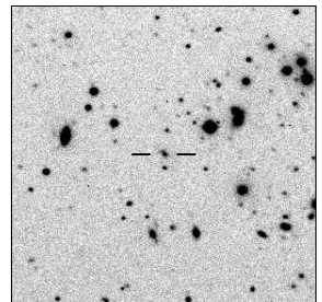
MRC B2319-550
