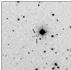
MRC B2259-375
