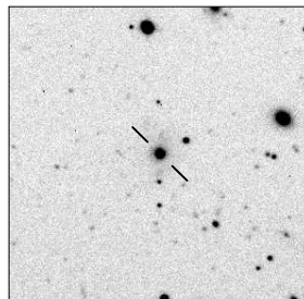
MRC B2153-699
