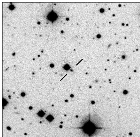
MRC B1953-425
