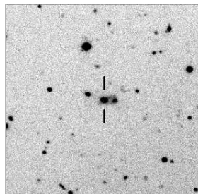
MRC B2250-412
