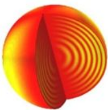
Fig. 1: Model of oscillation mode in a star.
