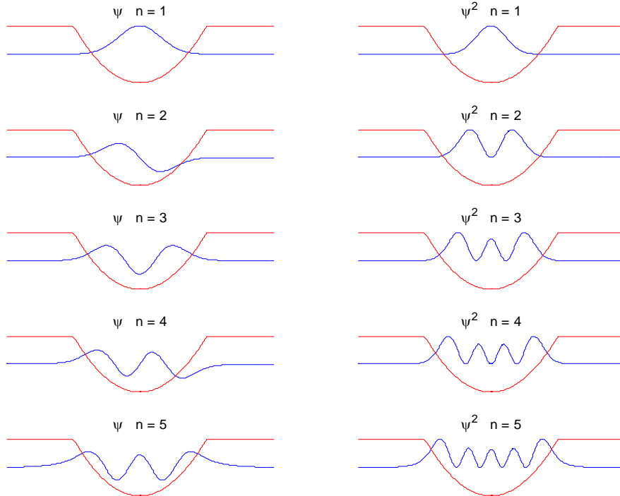
Fig. 17. The eigenfunctions and probability distributions for the harmonic oscillator.
