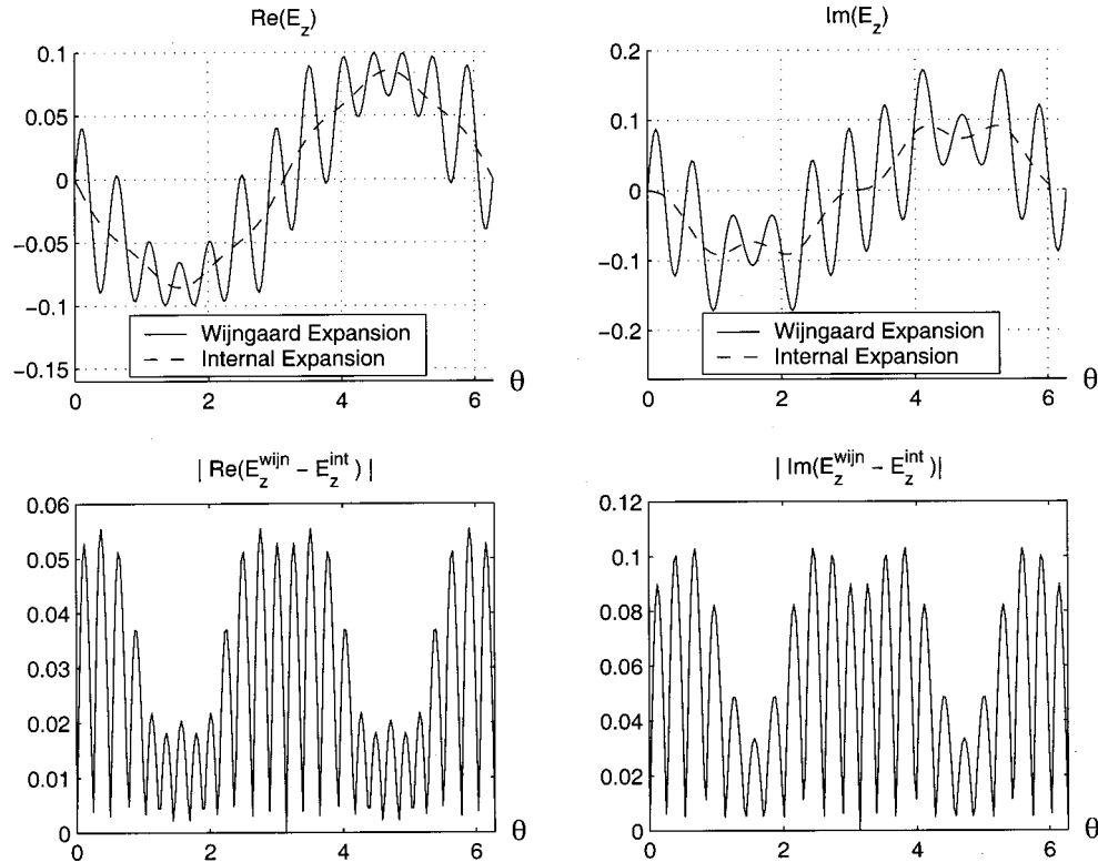
Fig. 1. Top, internal and bottom, Wijngaard expansions compared for \Re(E_z) and \Im(E_z) , respectively, for an air core MOF, with M = 5 for both the central air hole and all other air holes (3 rings; 54 air holes of diameter 4.0271 \mu\text{m} ; core hole diameter, 13.0714 \mu\text{m} ; jacket diameter, 50 \mu\text{m} ; n_e = 1.39 ; n_i = 1.00 ; n_0 = 1.39 + 10^{-8}i ; \Lambda = 5.78157 \mu\text{m} ; \lambda = 3.846 \mu\text{m} ).
