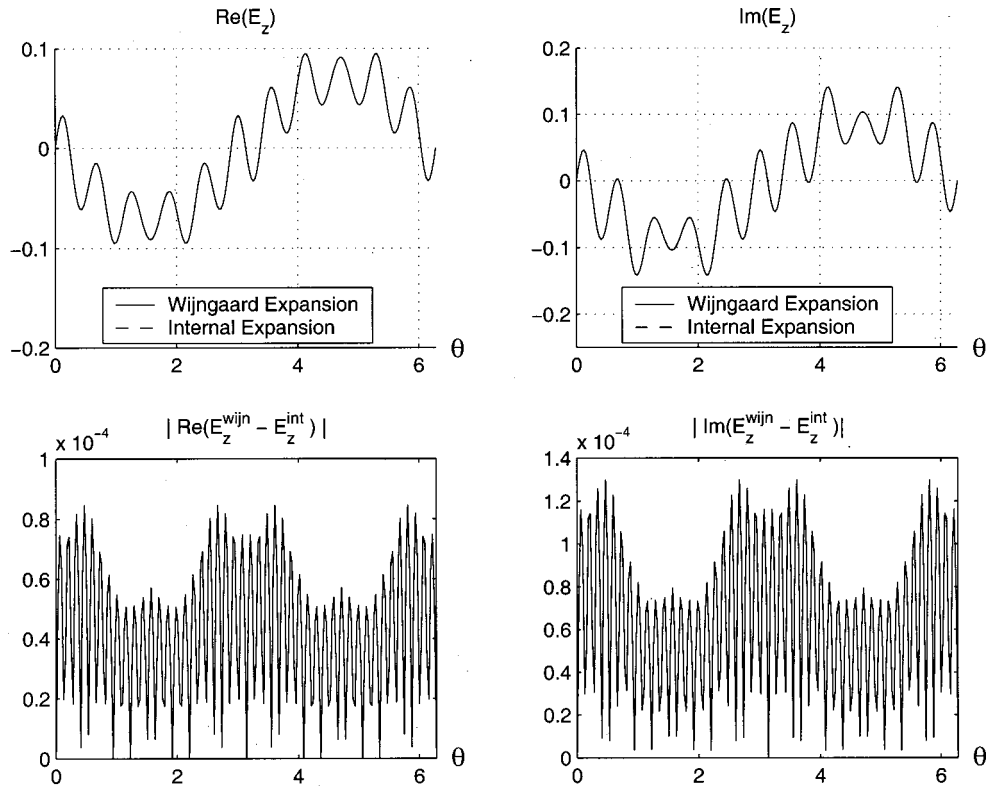
Fig. 2. As for Fig. 1 but with M = 19 for the core hole and M = 5 for all other holes. Note that the Wijngaard and internal expansions now match with graphic accuracy.
