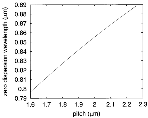
Fig. 10. Zero-dispersion wavelength as a function of pitch for the structure published by Kubota et al. , 3 with constant diameter/pitch ratio d/\Lambda = 0.67 .
