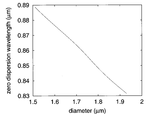
Fig. 9. Zero-dispersion wavelength as a function of hole diameter for the structure published by Kubota et al. , 3 with constant pitch \Lambda = 2.26 \mu\text{m} .
