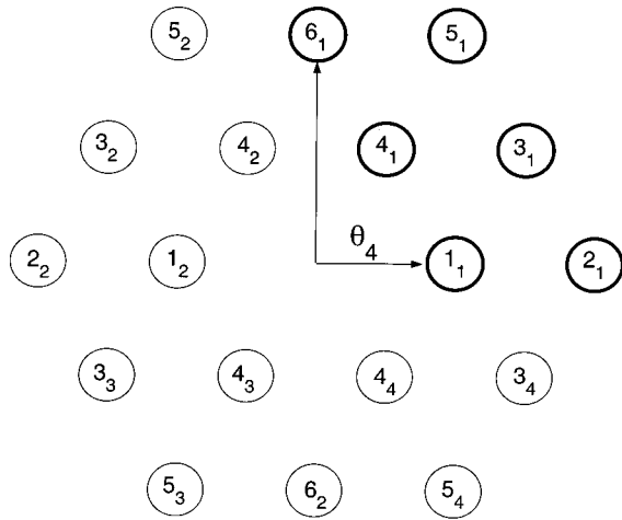
Fig. 12. Primary (bold circles) and secondary cylinders of the degenerate p = 3 and p = 4 mode classes of a two-ring MOF structure.
