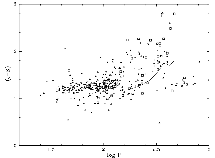
Fig. 12. \log P vs. (J - K) relation for AGAPEROS variables in the LMC. The line indicates the average colours of Sgr I Miras for various period groups (Glass et al. 1995). The symbols are the same as in Fig. 10.
