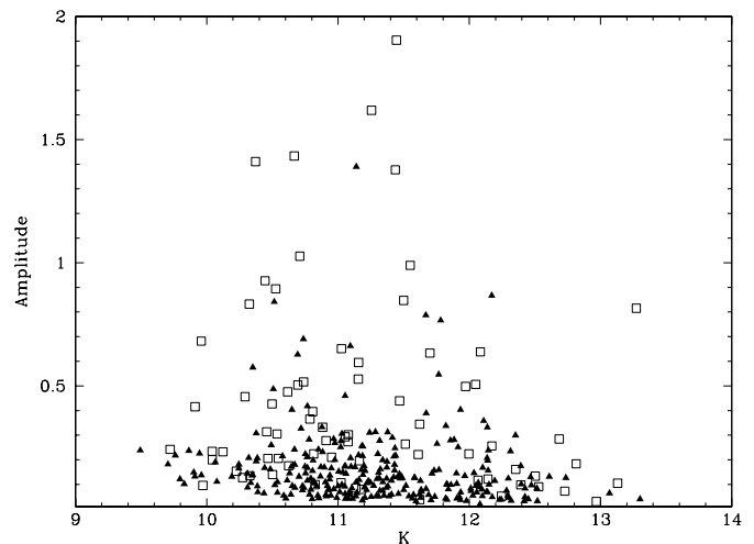
Fig. 15. R_{EROS} amplitude versus K_S . Open boxes denote regular variables, filled triangles semiregular stars.
