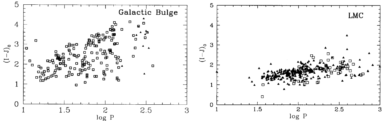
Fig. 11. Log P vs. (I - J) relation for MACHO variables in Baade’s window (Schultheis & Glass 2001) compared to AGAPEROS variables in the LMC. The open squares on the left panel indicate the SRVS, while the filled triangles the Mira variables. On the right panel, same symbols as in Fig. 10. The periods are given in days.
