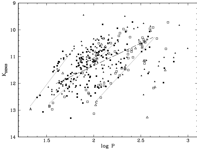
Fig. 13. K_S vs. \log P diagram for AGAPEROS variables. The dashed line is the relationship suggested for local SRVs by Bedding & Zijlstra (1998). The dotted lines labelled A, B and C are eye fits to the sequence by Wood (2000). We use only the primary periods. Open squares show regular variables with one single period while regular variables with a second period are shown as open triangles. Semiregular variables with one single period are shown as filled squares while those with their second period are indicated as filled triangles. Sequence D of Wood (2000) lies on the right-hand side.
