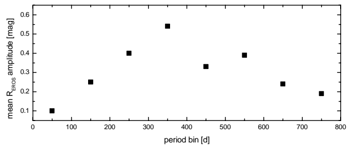
Fig. 6. Mean amplitude for each period bin. Only the primary period has been used in this plot.
