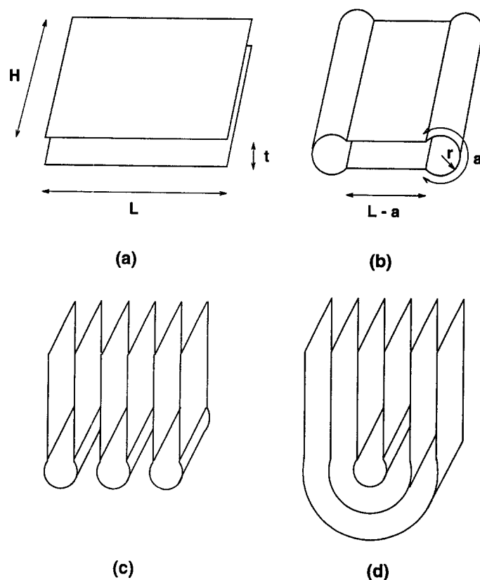
Fig. 3. Diagrams showing: (a) a two-layer structure with dangling edges and (b) joining two of its parallel sides via open tubules; (c)–(d) extension of (b) to six layers, indicating two possibilities of terminating one side of the dangling edges.
