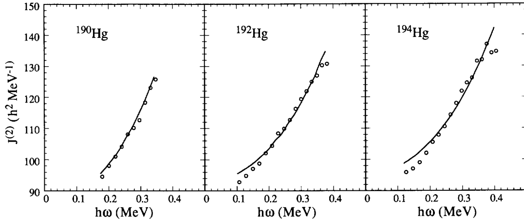
Fig. 3. Comparison of the experimental dynamic moment of inertia in ^{190-194}\text{Hg} (circles) with the super IBM calculations (solid lines). The data are from [13]. The parameters used in the fits are N_{\text{super}} = 29, 30, 31 , \kappa = -35, -34, -33 keV, q = 0.68, 0.72, 0.72 for ^{190-192-194}\text{Hg} , respectively.
