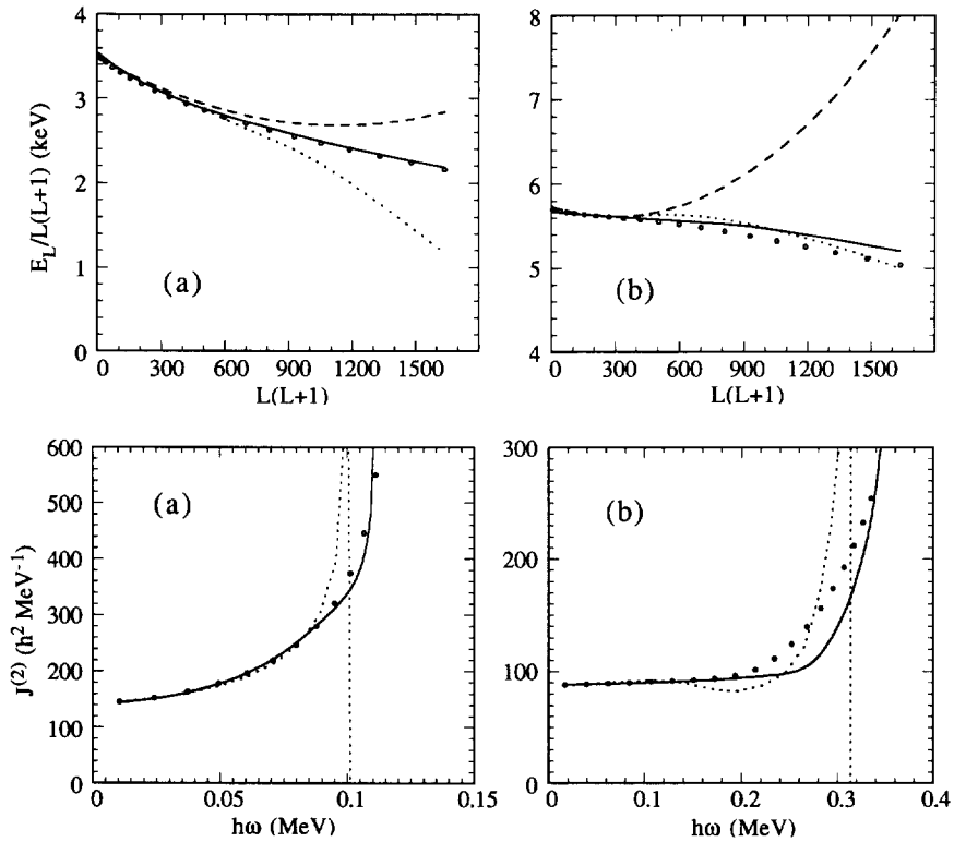
Fig. 1. Comparison of the ground band energies (top) and dynamic moments of inertia (bottom) obtained from the 1/N expansion with the exact numerical results (circles). The different lines refer to the third layer calculation with VAP (solid line), third layer with VBP (dashed line), and second layer with VAP (dotted line). The VBP results for \mathcal{J}^{(2)} deviate strongly from the exact ones and are not shown to avoid cluttering of the figures. The parameters of H are \kappa = -20 keV, q = 0.7 for the quadrupole interaction in both (a) and (b), and \varepsilon_g = 500 keV in (b).
