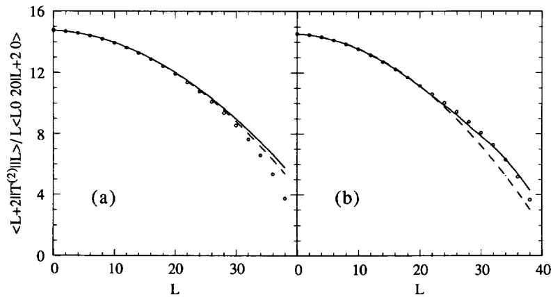
Fig. 2. Comparison of the E2 transition m.e., Eq. (12) with the exact diagonalization results (circles). Solid line refers to VAP and dashed line to VBP.
