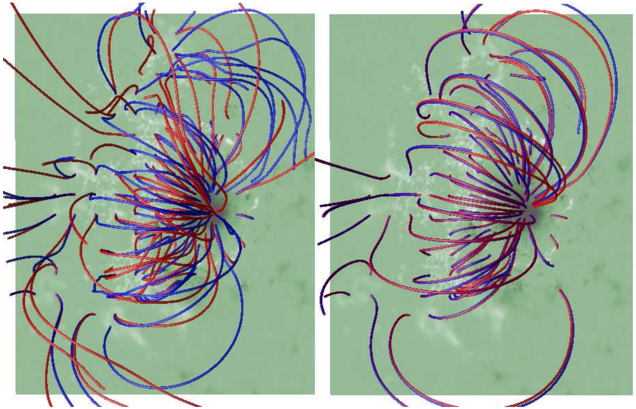
Fig. 1.— Left panel: Overlay of field lines for the two force-free solutions constructed using boundary conditions on current density taken from the positive polarity (blue lines), and from the negative polarity (red lines), using the original boundary data (solutions k = 1 and k = 2 ). Right panel: Overlay of the field lines for the two solutions after 10 self-consistency cycles (solutions k = 19 and k = 20 ). The image in the background of each panel shows the boundary values of B_z , with positive polarity areas appearing light, and negative polarity areas dark. See the electronic edition of the Journal for a color version of this figure.
