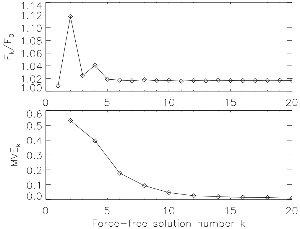
Fig. 2.— Upper panel: The magnetic energy E_k of each force-free solution, in units of the energy of the potential field E_0 , over the 10 self-consistency cycles. Solutions k = 1, 3, \dots, 19 are constructed using \alpha values on the positive polarity, and solutions k = 2, 4, \dots, 20 using values on the negative polarity. Lower panel: The mean vector error, quantifying the discrepancy between the two fields constructed at each cycle.
