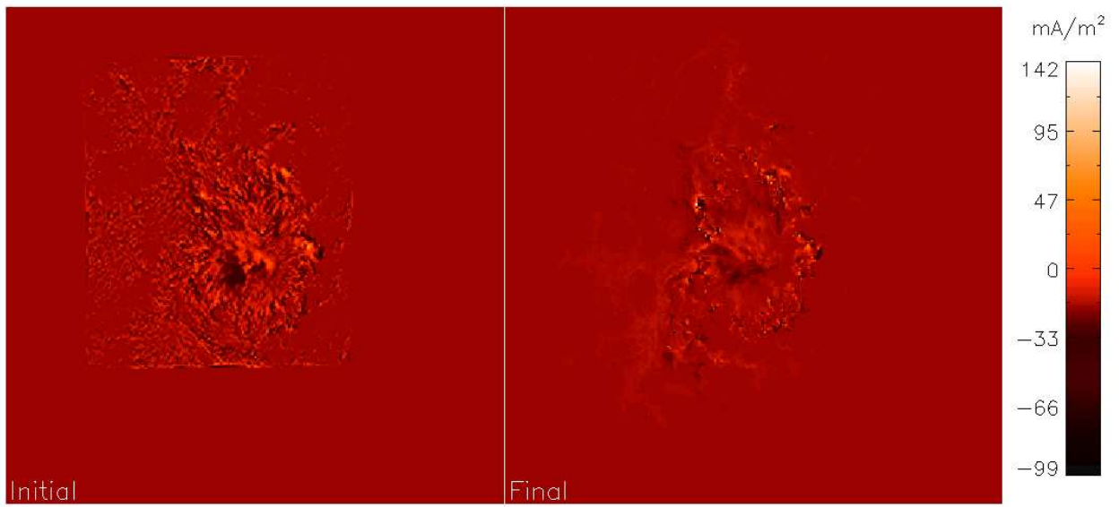
Fig. 3.— Boundary conditions on electric current density in the observations (left panel) and in the solution after 10 self-consistency cycles (right panel).
