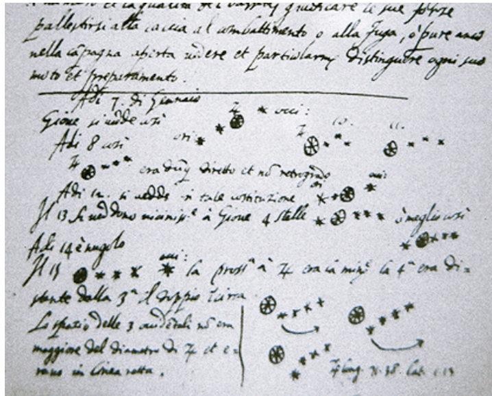
Part of Galileo's journal from 1610, with sketches of the four "stars" near Jupiter which he later recognized to be moons.
