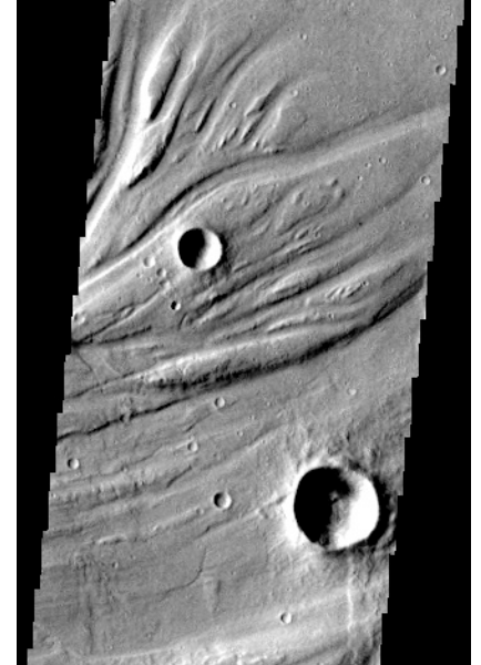
Outflow in Chryse Planitia, about 20 km across. The crater at the top pre-dates the flow, while the bottom craters post-date it.
