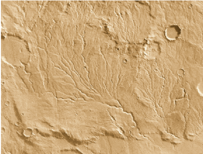
Network of drainage channels, suggesting sustained flows of water.
