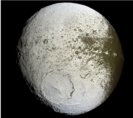
The extreme brightness dichotomy of Iapetus.
