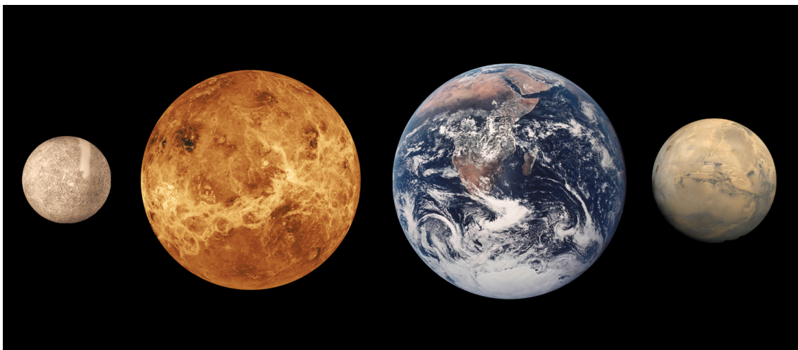
71 The four terrestrial planets: Mercury, Venus, Earth and Mars, showing the relative sizes.
