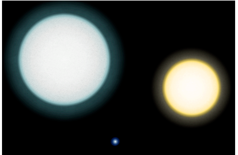
Size of the white dwarf IK Pegasi B (center) compared to its A-class companion IK Pegasi A (left) and the Sun (right).
