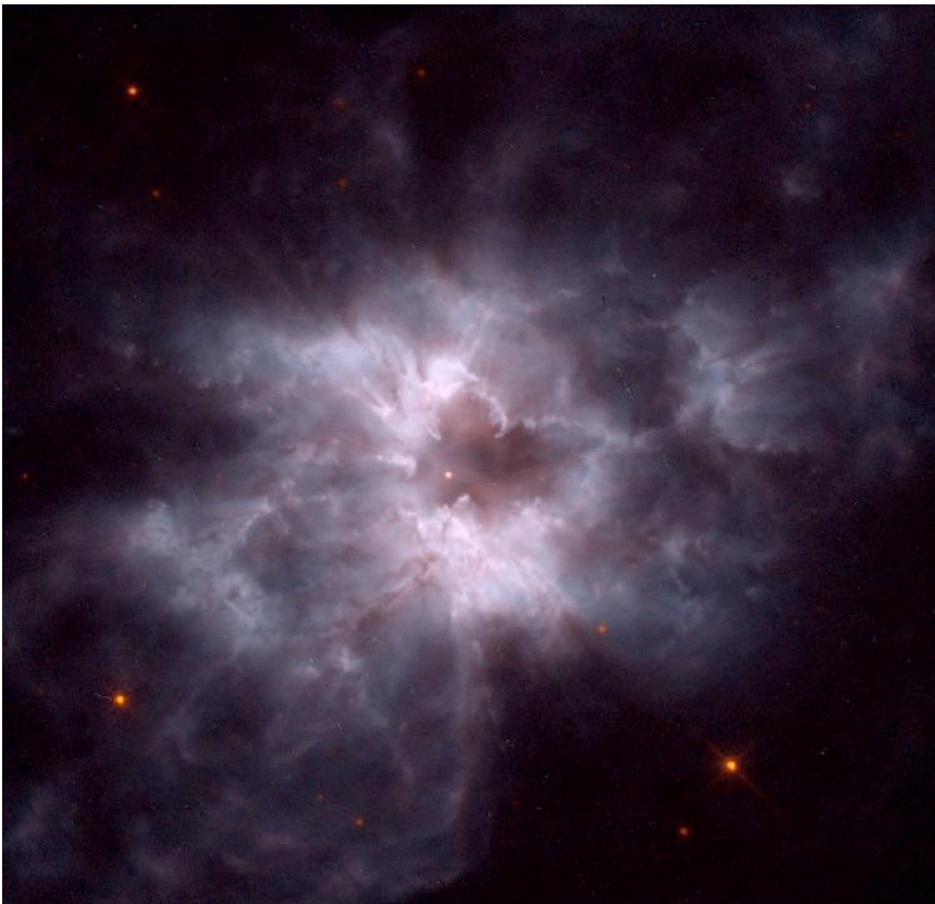
HST image of NGC 2440; the white dwarf, visible at the centre, is one of the hottest white dwarf stars known.
