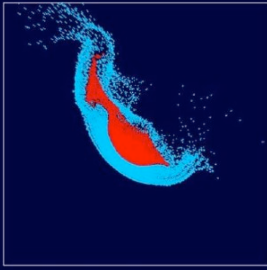
GIANT IMPACT ON PROTO-MERCURY t = 8.22 \text{ min} / [-3.5, 2.5, -3, 3]
