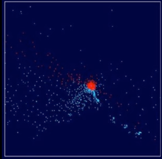
GIANT IMPACT ON PROTO-MERCURY t = 194.35 \text{ min} / [-7, 21, -20, 8]
