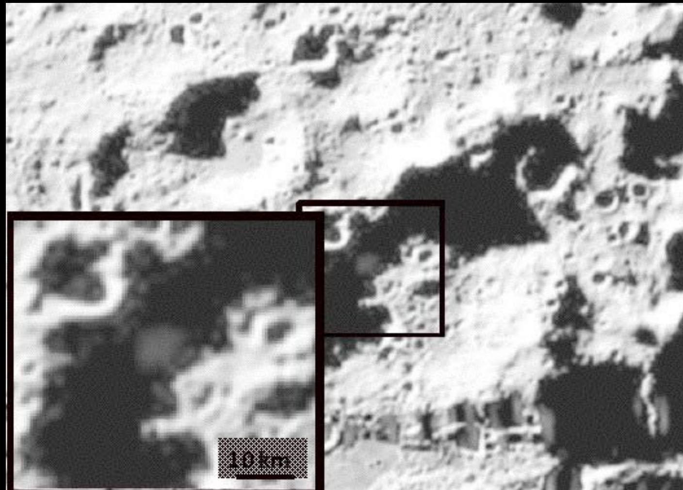
LCROSS image of the ejecta plume
