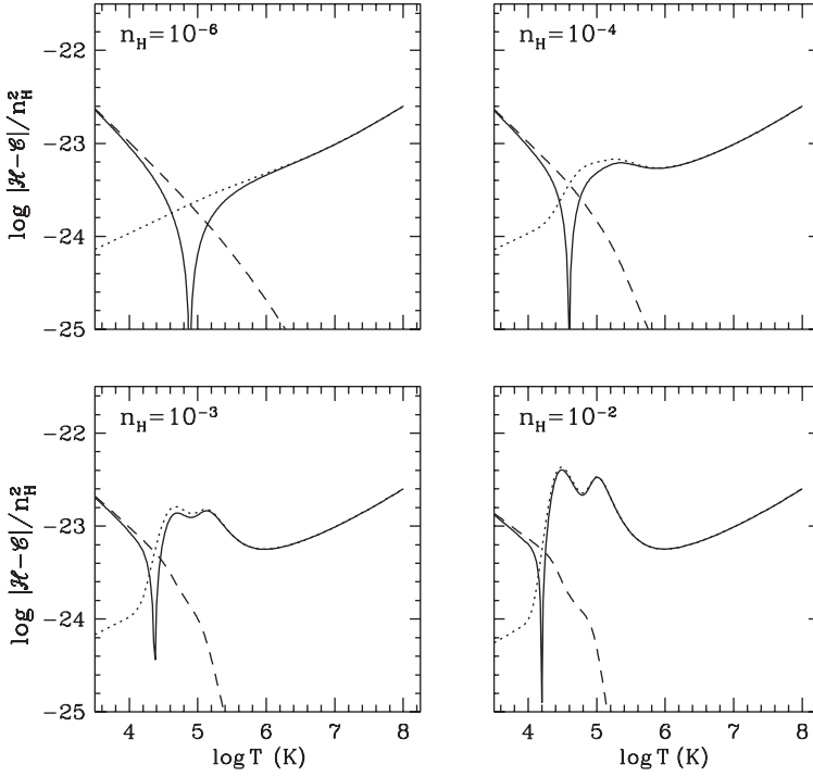
Fig. 8.2. Net cooling rates as a function of temperature for a gas of primordial composition in ionization equilibrium with a UV radiation background of intensity J(\nu) = 10^{-22}(\nu_H/\nu) \text{ erg s}^{-1} \text{ cm}^{-2} \text{ sr}^{-1} \text{ Hz}^{-1} . Results are shown for four different hydrogen number densities n_H = 10^{-6}, 10^{-4}, 10^{-3} , and 10^{-2} \text{ cm}^{-3} , as indicated. In each panel, the dotted line shows the cooling rate and the dashed line shows the rate of heating by photoionization. The solid curve shows the absolute value of the net cooling rate (in \text{erg cm}^3 \text{ s}^{-1} ); heating dominates at low temperatures and cooling at high temperatures. [Adapted from Weinberg et al. (1997a) by permission of AAS]
