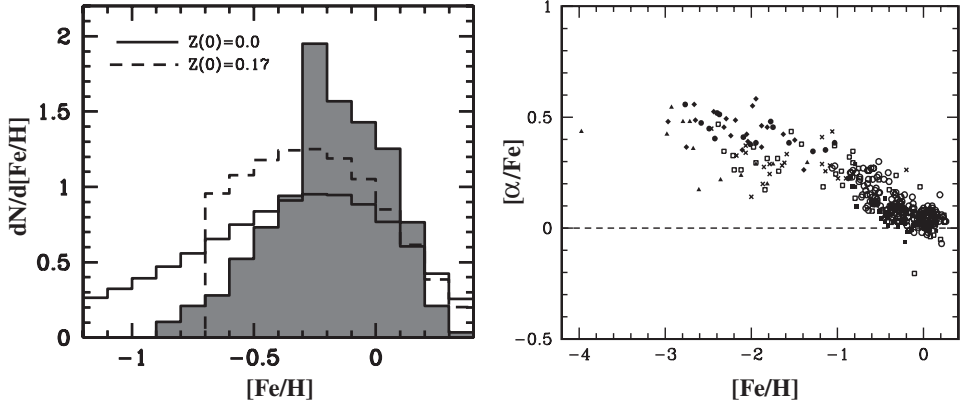
Fig. 11.8. Left panel: The shaded histogram shows the metallicity distribution of G-dwarfs in the solar neighborhood (data taken from Rocha-Pinto & Maciel, 1996). For comparison, we also show two predictions of closed-box models with initial metallicities of Z(0) = 0 and Z(0) = 0.17 , as indicated. Right panel: Abundance ratios of stars as a function of metallicity, based on data published in Edvardsson et al. (1993, open circles) and Wheeler et al. (1989, other symbols).
