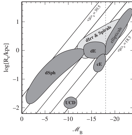
Fig. 2.24. A sketch of the regions in the parameter space of effective radius and absolute magnitude (both in the B -band) occupied by different types of galaxies. The spheroidal systems are split into ellipticals, dwarf ellipticals (dE), compact ellipticals (cE), dwarf spheroidals (dSph), and ultra-compact dwarfs (UCD). The dashed, vertical line corresponds to M_B = -18 , and reflects the magnitude limit below which galaxies are often classified as dwarfs. The diagonal lines are lines of constant surface brightness; galaxies roughly span five orders of magnitude in surface brightness, from \langle\mu_B\rangle_e \sim -18.5 to \langle\mu_B\rangle_e \sim -30.5 .
