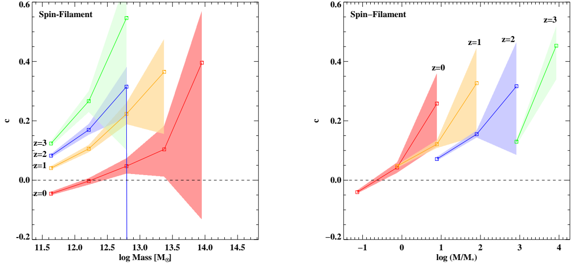
FIG. 4.— The alignment of dark matter halo spin with filaments over cosmic time. Alignment is characterized by the parameter c of the fit of Equation 12 to the distribution of |\cos \theta| , where positive c indicates parallel alignment and negative c indicates orthogonal alignment. At high redshift all spins are orthogonal to filaments but recent times, low mass haloes have a parallel alignment with filaments. The dashed line is the expected distribution for random halo spins and the shaded regions are the 1\sigma errors. The red line is for z=0 , yellow line is z=1 , blue is z=2 and green line is z=3 . The alignment is shown for haloes in bins of halo mass (left) and halo mass normalized by the characteristic mass (right).
